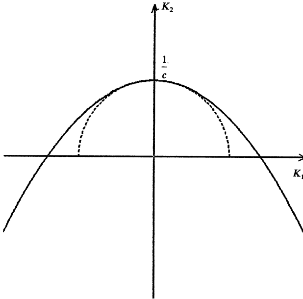
FIG. 2.1. Dispersion relations.
