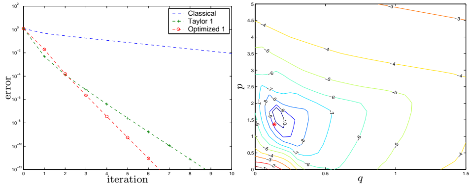
FIGURE 5. Left: convergence curves of the classical Schwarz waveform relaxation algorithm with Dirichlet transmission conditions compared to the same algorithm with the new first order transmission conditions. Right: the error obtained running the algorithm with first order transmission conditions for 5 steps and various choices of the free parameters p and q , and indicated by a star the choice p^* , q^* predicted by the theory.
