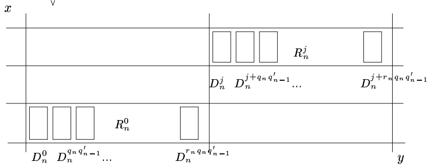
Fig. 1. The rational rotation.
