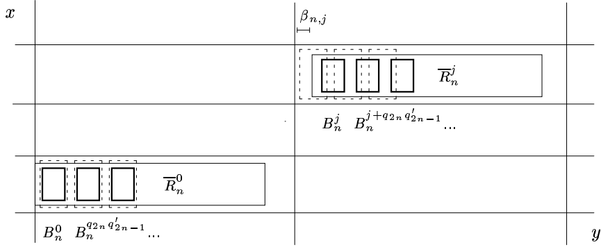
Fig. 2. The special tower of R_{\alpha, \alpha'} .
