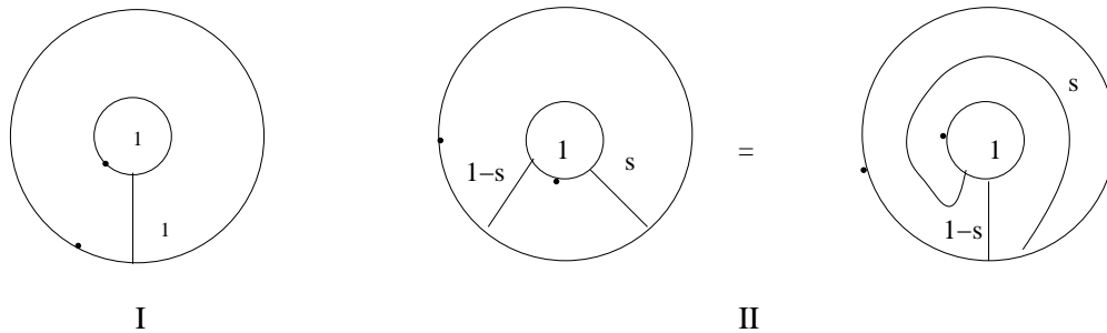
Figure 6: I, the identity and II, the arc family \delta yielding the BV operator
