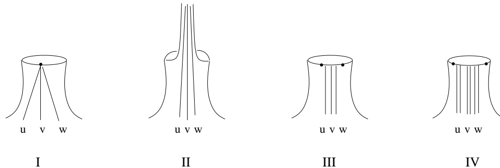
Figure 2: I, arcs running to a point on the boundary, II, arcs running to a point at infinity, III, arcs in a window, IV, bands in a window
