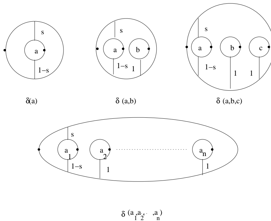
Figure 9: The definition of the n -ary operations \delta
