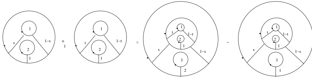
Figure 13: The first iterated gluing of \ast
