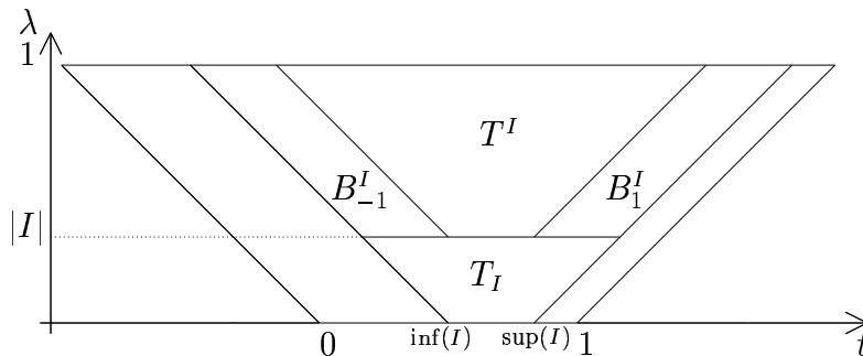
Figure 1 : Illustration of the sets in H defined early.
