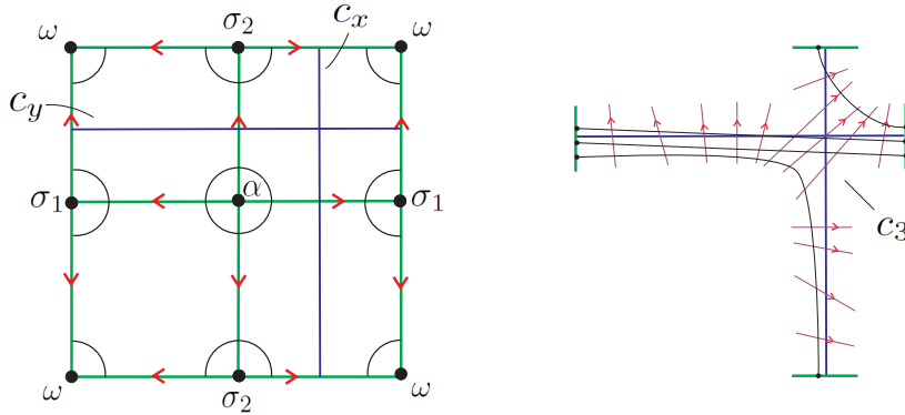
Figure 18: The curves c_x , c_y and c_3
