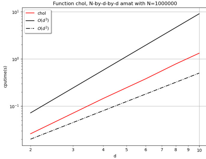
Figure 3: Computational times in seconds of B=chol(A) where A is a N -by- d -by- d symmetric positive definite amat object.
