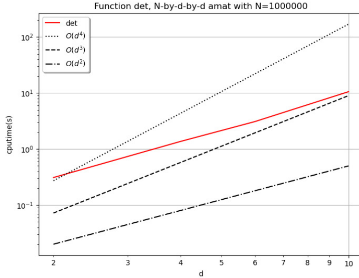
Figure 4: Computational times in seconds of \mathbf{B}=\text{det}(\mathbf{A}) where \mathbf{A} is a N -by- d -by- d amat object.
