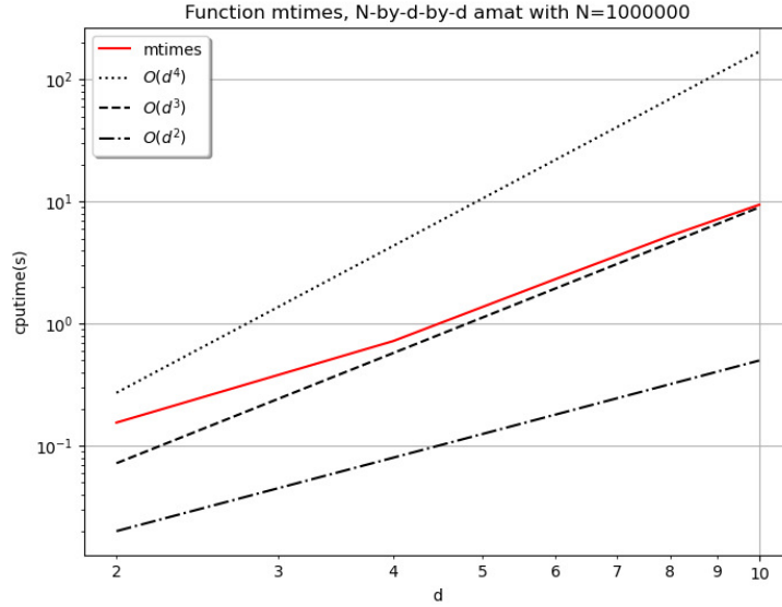
Figure 1: Computational times in seconds of mtimes(X,Y) or \mathbf{X}*\mathbf{Y} (matrix product) where \mathbf{X} and \mathbf{Y} are N -by- d -by- d amat objects.
