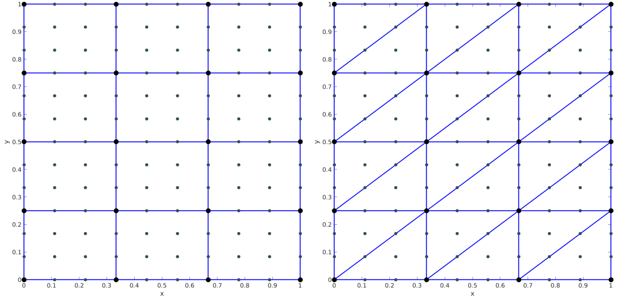
Figure 5: Tessellation samples of [0, 1]^2 with 3-order 2-orthotopes (left) and 3-order 2-simplices (right) where nodes of all mesh elements are represented by black (vertices) and grey points.
