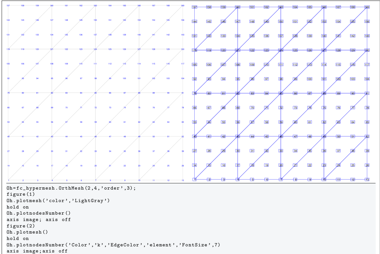
Listing 9: plotnodesNumber method of a 2D ElMesh objects , figure(1) (left) and figure(2) (right)
