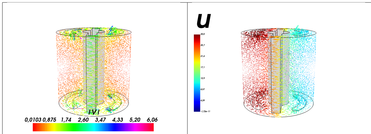
Figure 5.10: Potential flow \mathbf{V}
