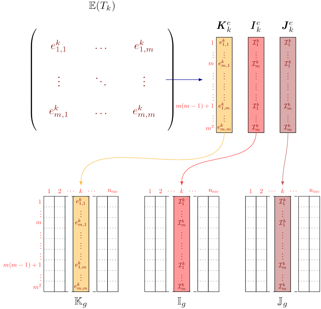
Figure 1.3: Construction of \mathbb{K}_g , \mathbb{I}_g and \mathbb{J}_g with loop
