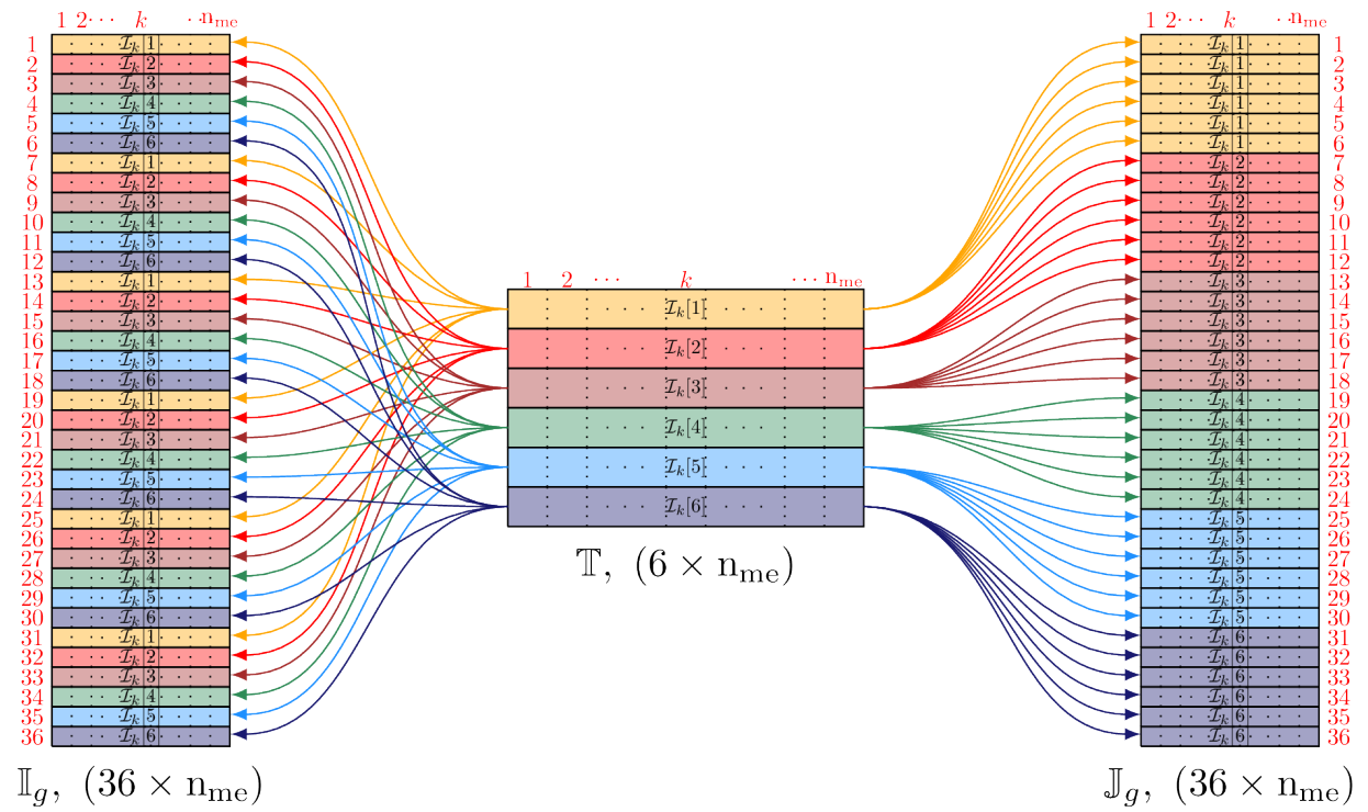
Figure 1.8: Construction of \mathbb{I}_g and \mathbb{J}_g : OptV2 version in 2d vector fields case
