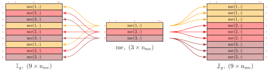
Figure 1.5: Construction of \mathbb{I}_g and \mathbb{J}_g : OptV2 version for 2d scalar matrix
