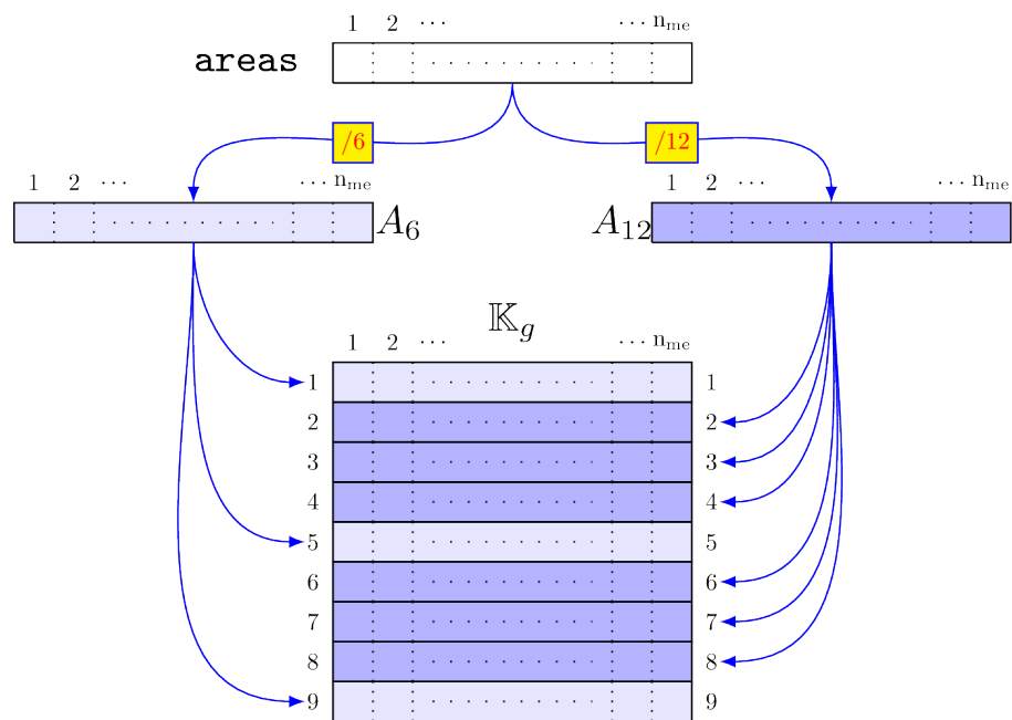
Figure 1.10: Construction of \mathbb{K}_g for Mass matrix
