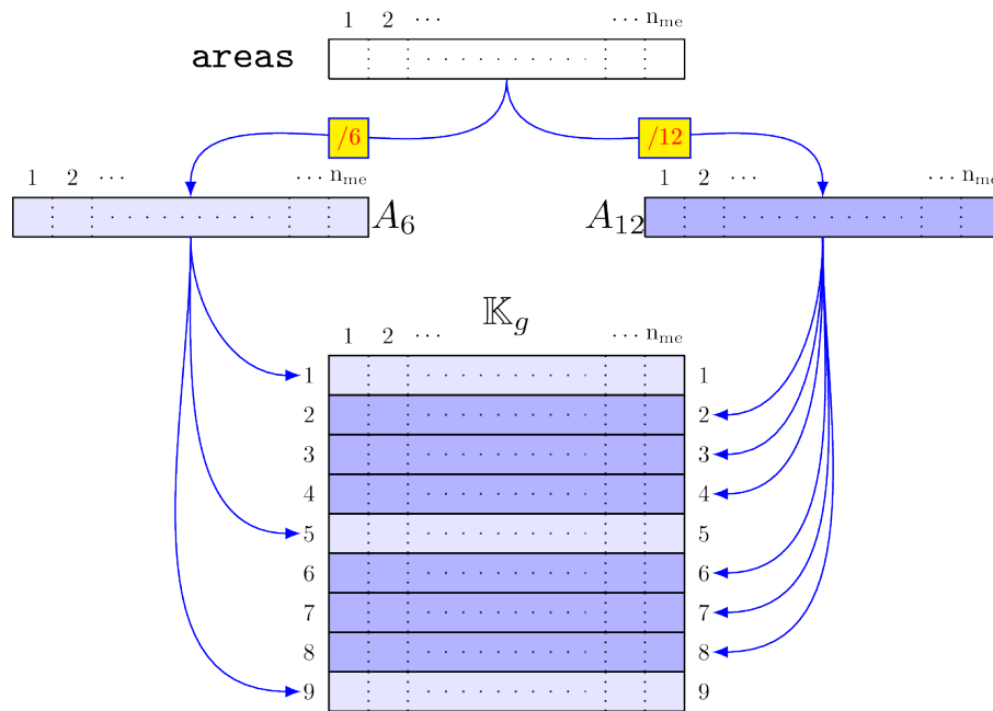
Figure 4.5: Construction of \mathbb{K}_g associated to 2d Mass matrix in
