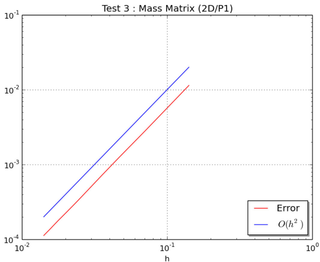
Figure 6.1: Graphical results of validMass2DP1-Test 3
