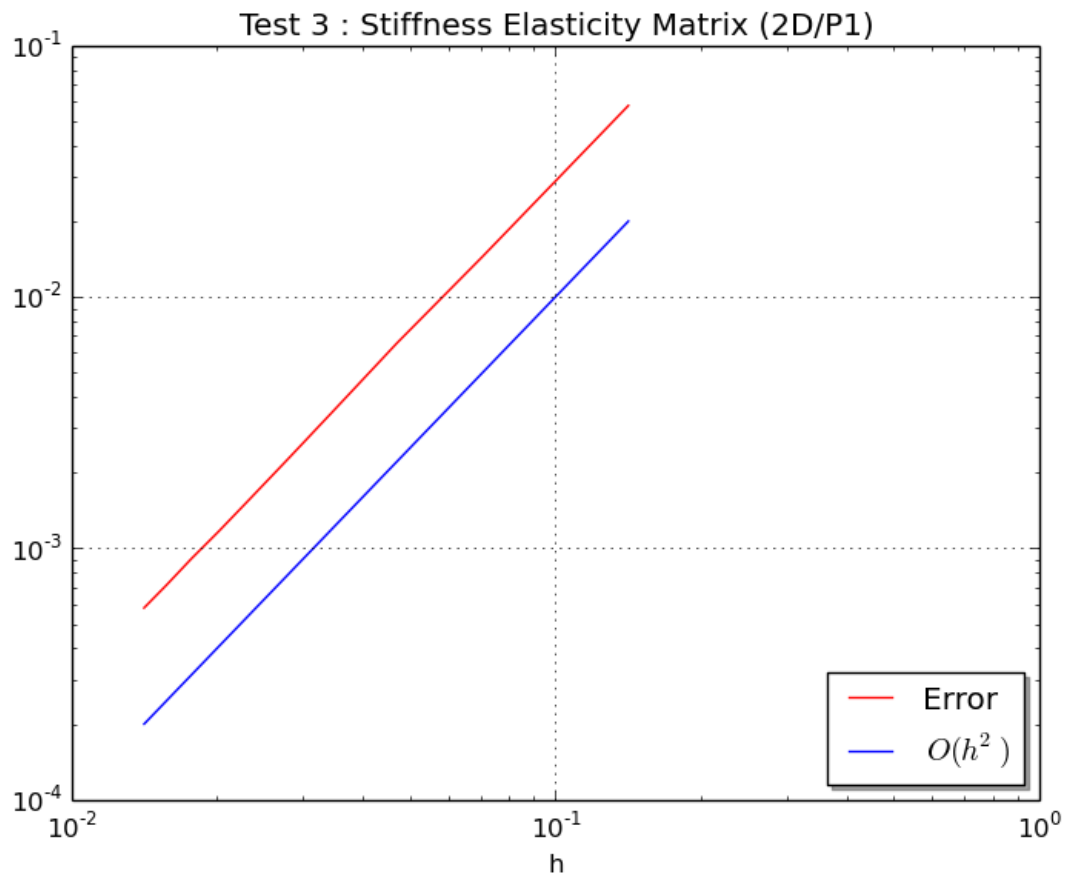
Figure 6.3: Graphical results of validStiffElas2DP1-Test 3
