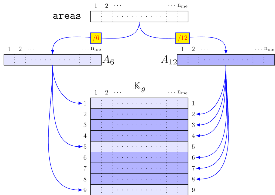
Figure 1.10: Build \mathbb{K}_g for Mass matrix
