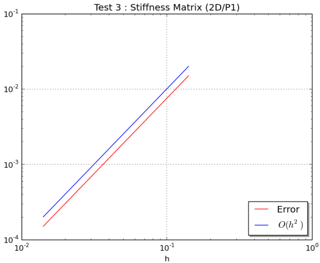
Figure 6.2: Graphical results of validStiff2DP1-Test 3
