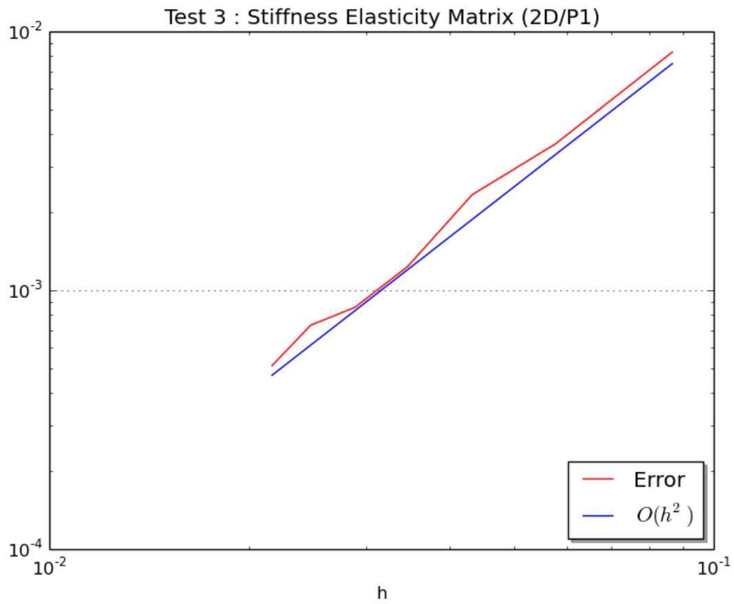
Figure 7.3: Graphical results of validStiffElas3DP1-Test 3
