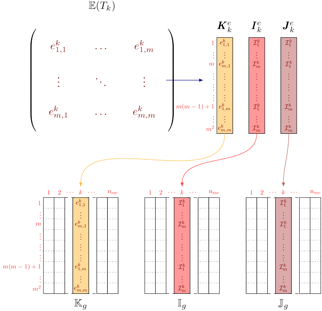
Figure 1.3: Build \mathbb{K}_g , \mathbb{I}_g and \mathbb{J}_g with loop
