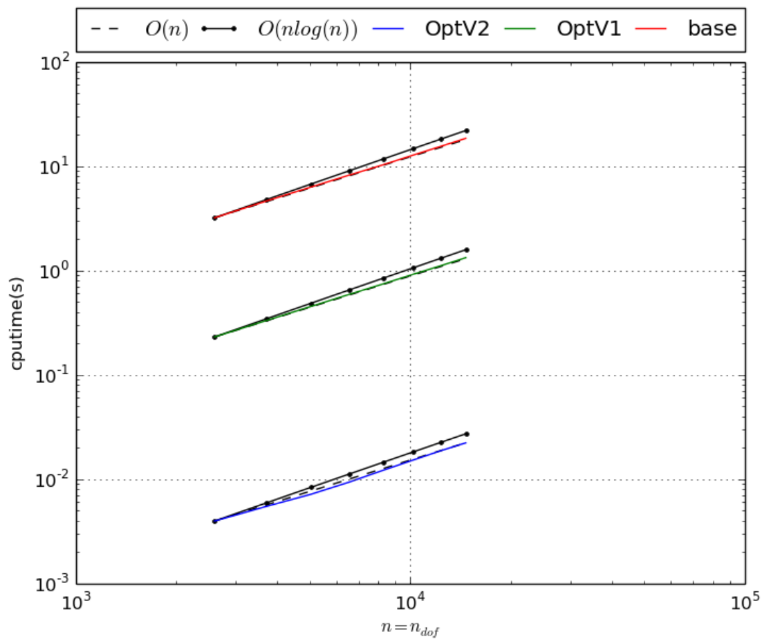
Figure 2.3: StiffAssembling2DP1 benchmark
