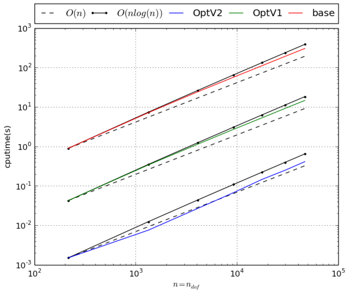
Figure 3.1: MassAssembling3DP1 benchmark
