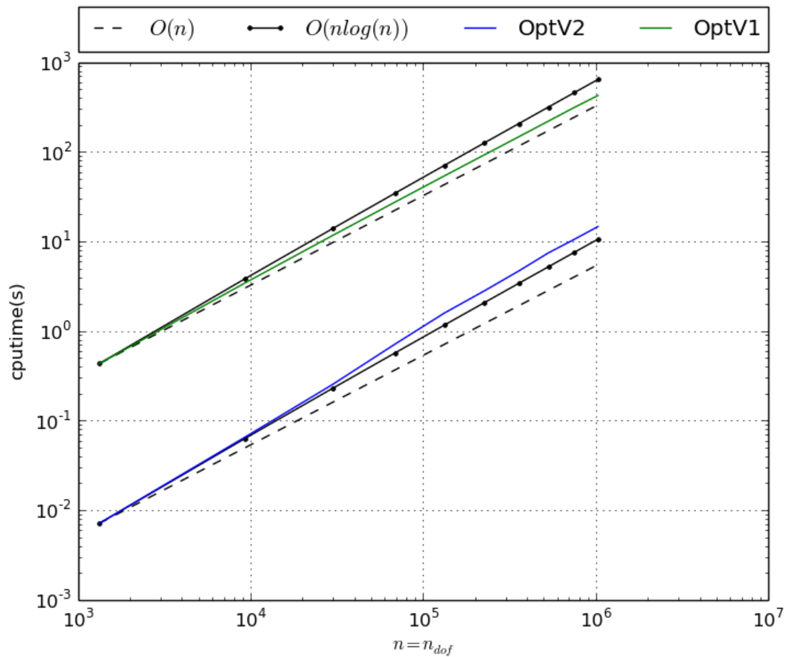
Figure 3.4: StiffAssembling3DP1 benchmark
