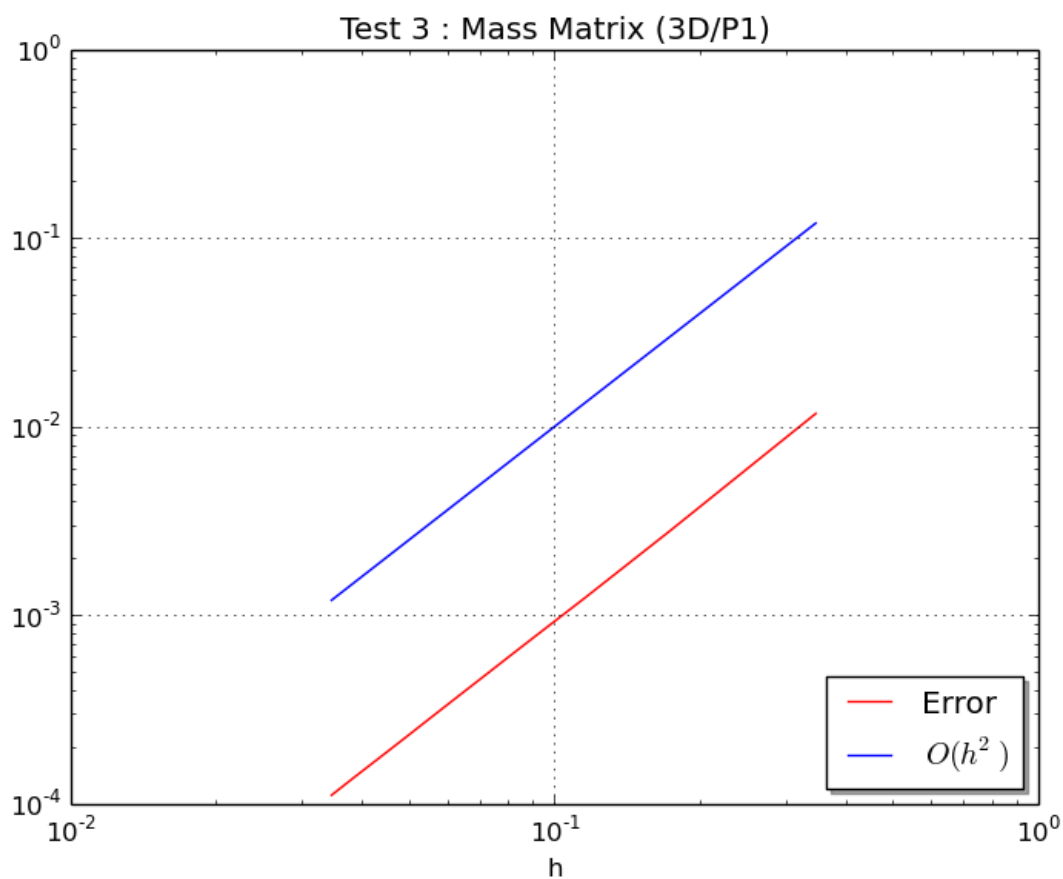
Figure 7.1: Graphical results of validMass3DP1-Test 3
