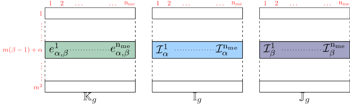
Figure 1.4: Row-wise operations on global arrays \mathbb{I}_g , \mathbb{J}_g and \mathbb{K}_g
