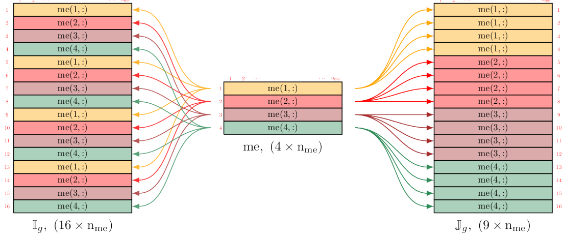
Figure 1.6: Build I_g and J_g : OptV2 version for 3d scalar matrix
