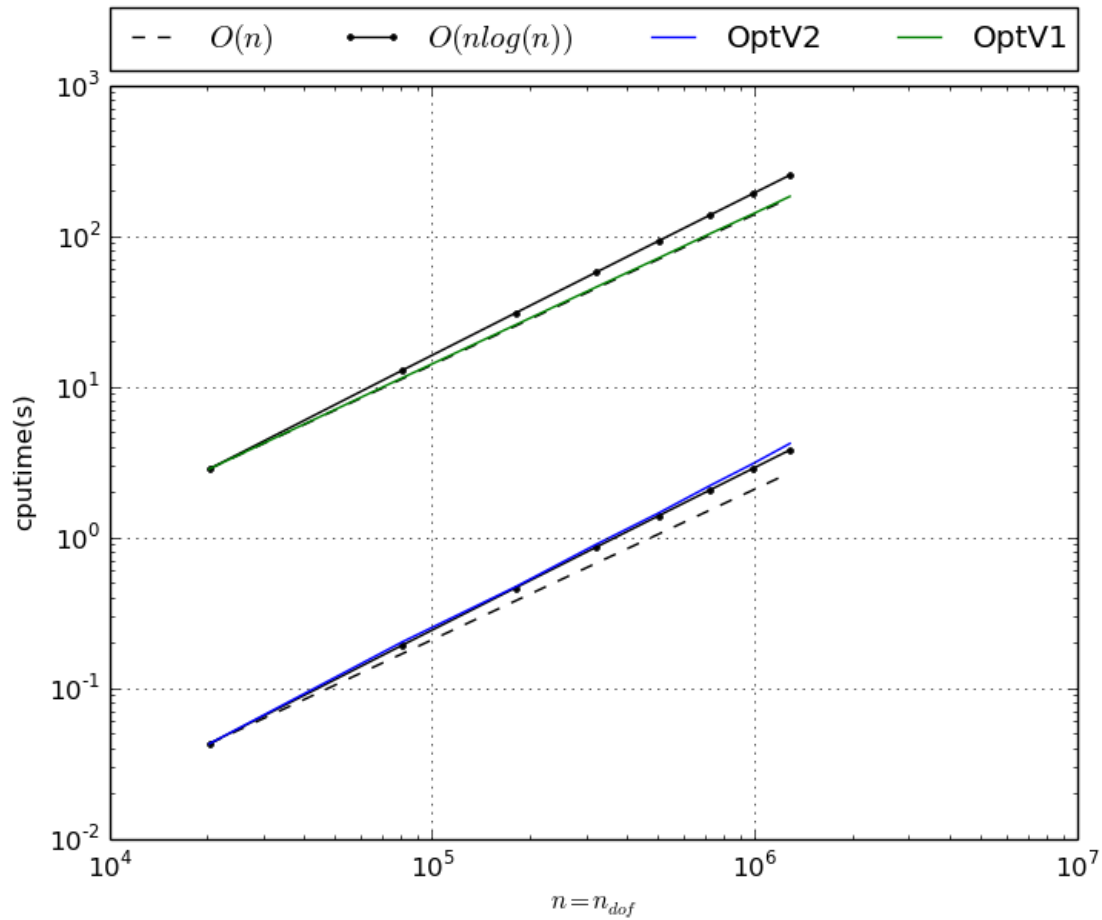
Figure 2.6: StiffElasAssembling2DP1 benchmark
