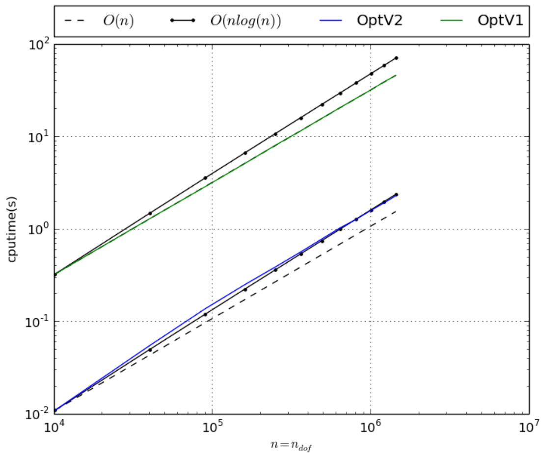
Figure 2.2: MassAssembling2DP1 benchmark
