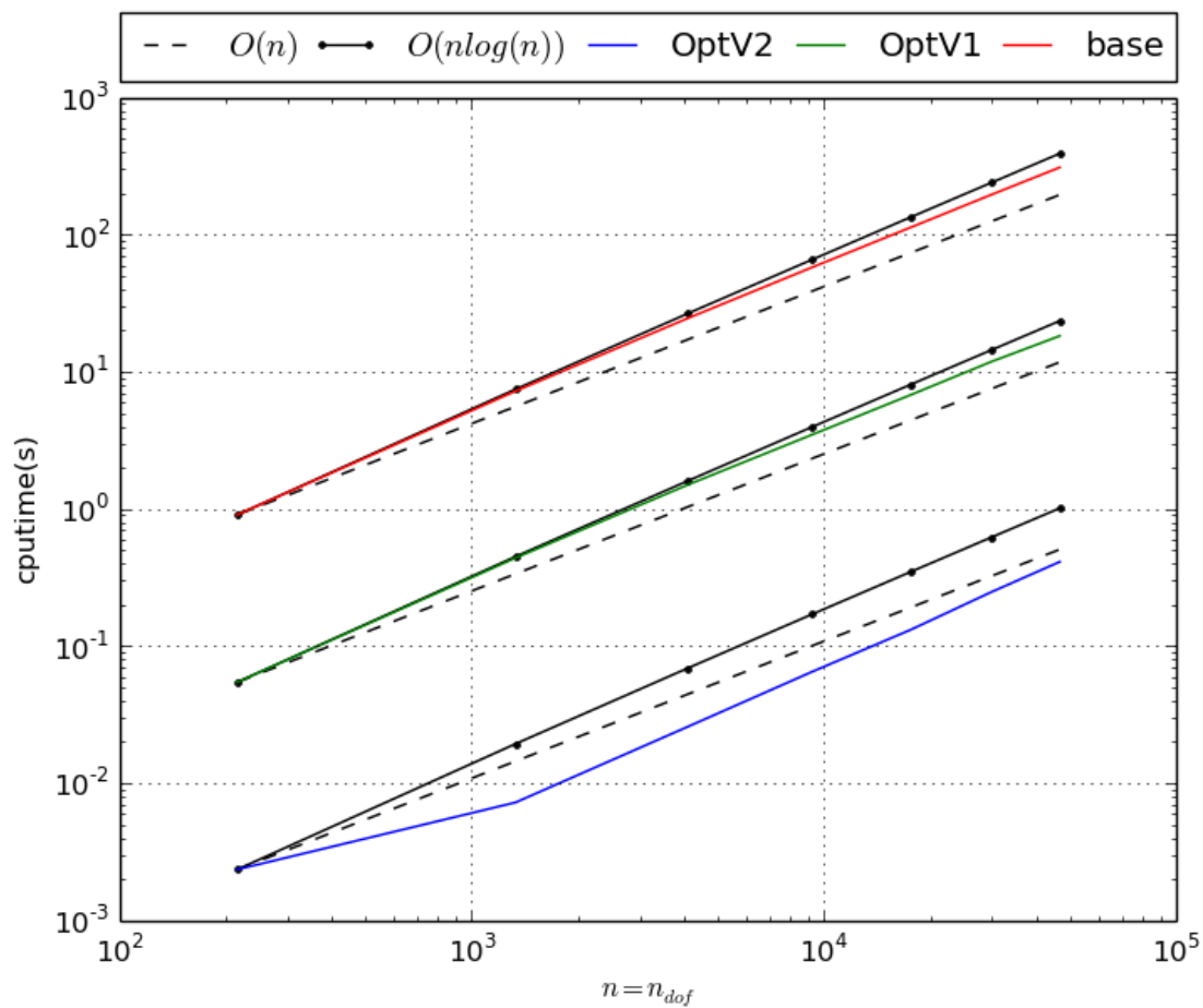
Figure 3.3: StiffAssembling3DP1 benchmark
