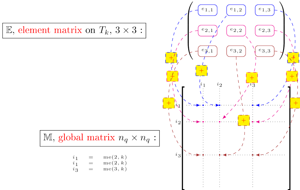
Figure 1.2: Adding of an element matrix to global matrix in 2d scalar fields case
