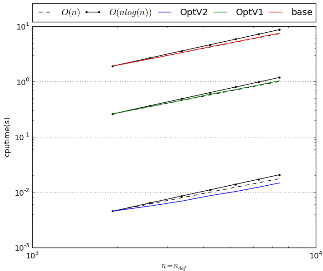
Figure 2.5: StiffElasAssembling2DP1 benchmark
