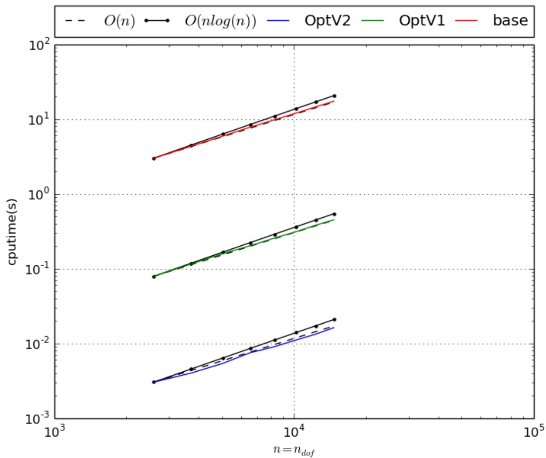
Figure 2.1: MassAssembling2DP1 benchmark
