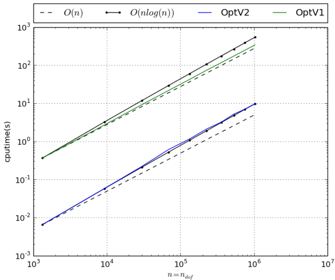
Figure 3.2: MassAssembling3DP1 benchmark
