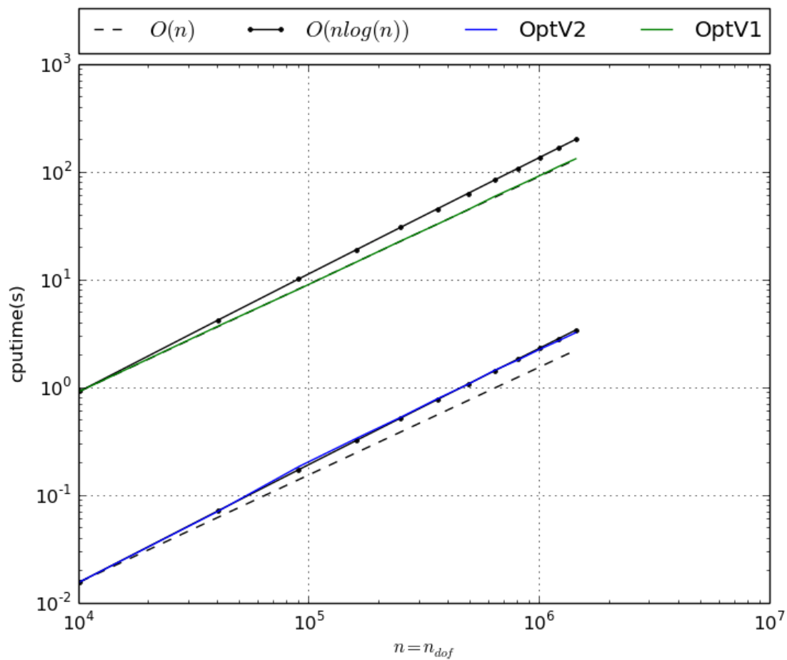
Figure 2.4: StiffAssembling2DP1 benchmark
