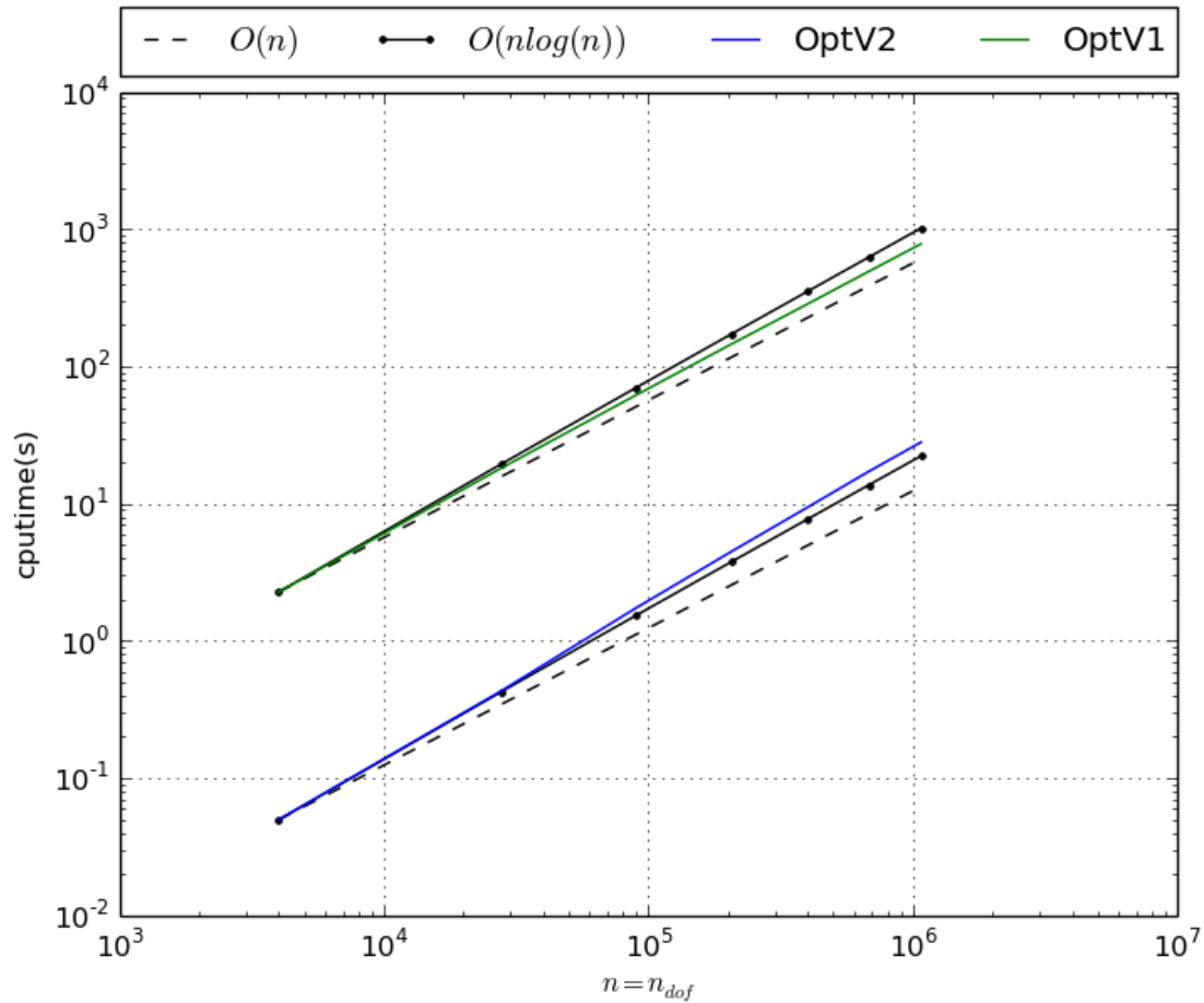
Figure 3.6: StiffElasAssembling3DP1 benchmark
