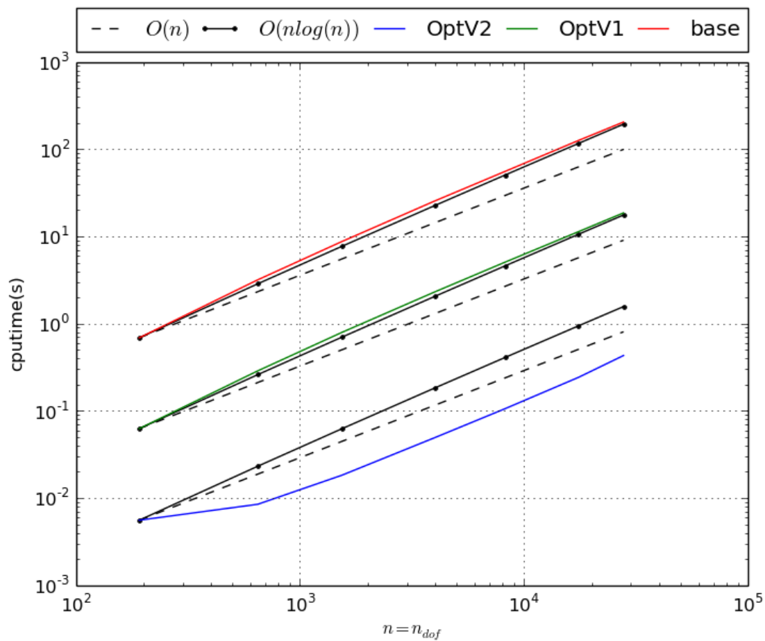
Figure 3.5: StiffElasAssembling3DP1 benchmark
