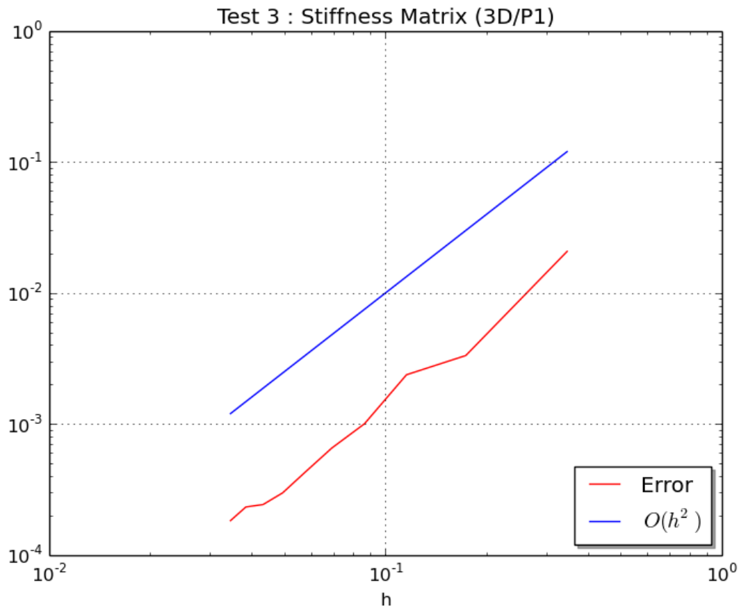
Figure 7.2: Graphical results of validStiff3DP1-Test 3
