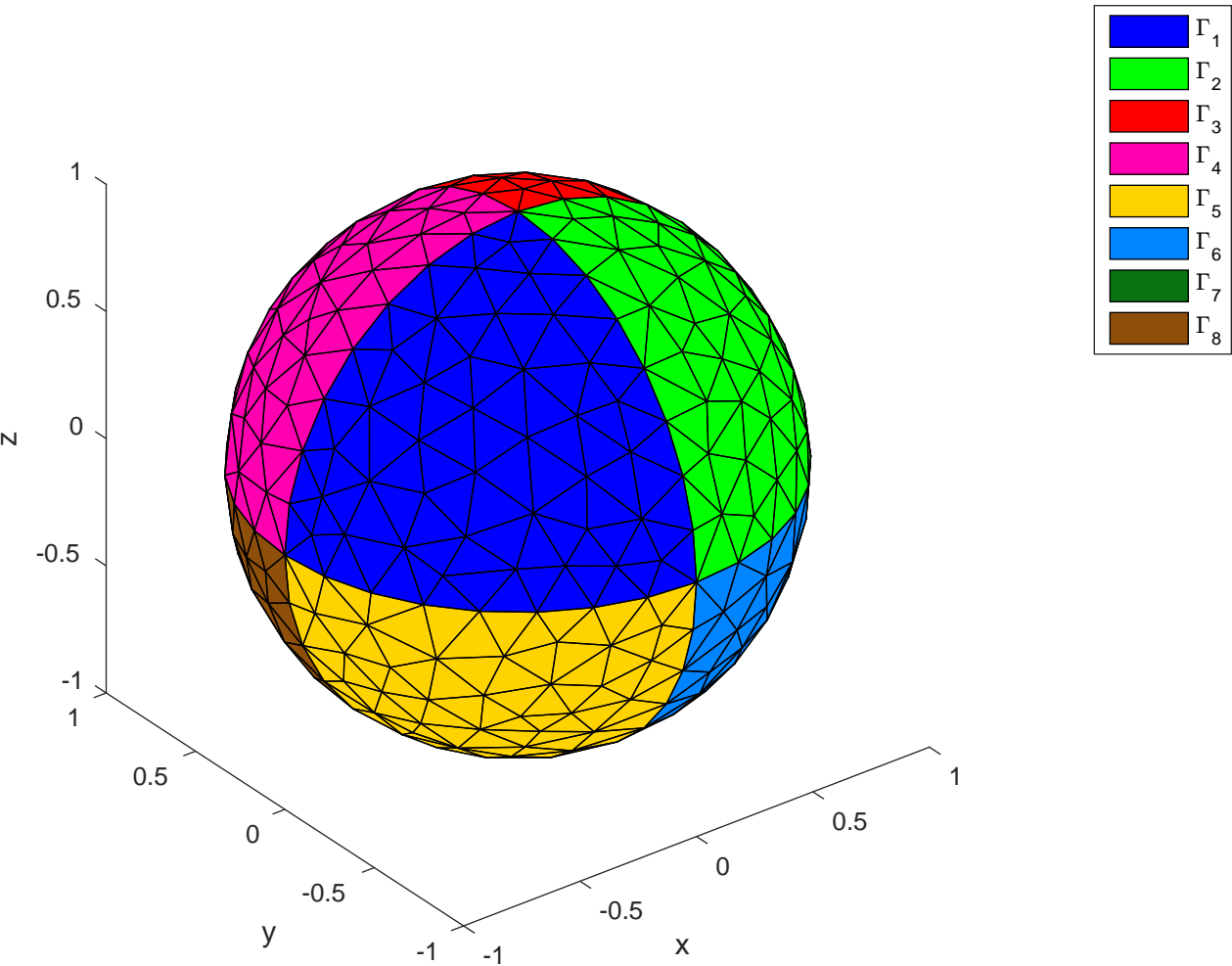
Boundaries of the mesh (ball8.geo)
