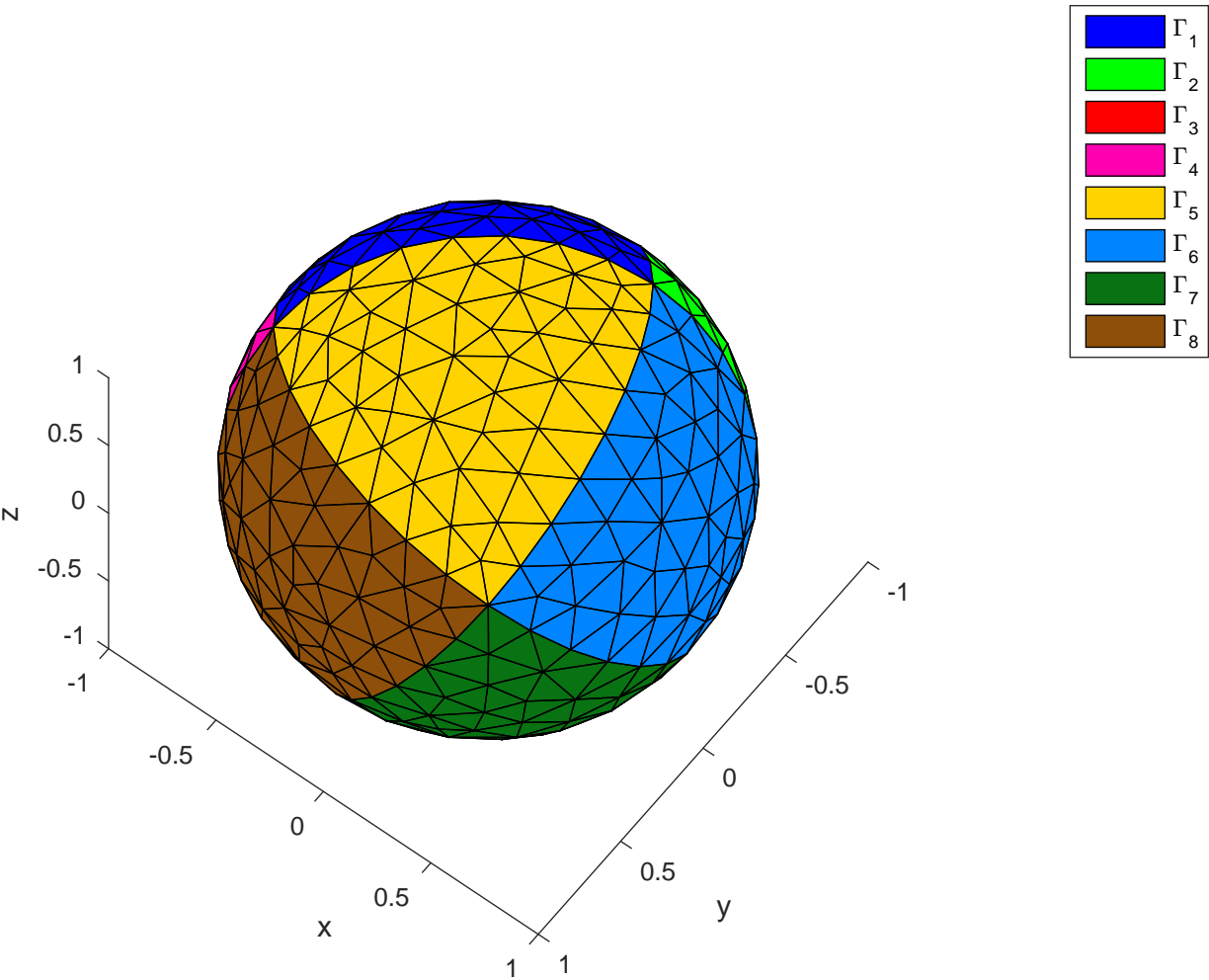
Boundaries of the mesh (ball8.geo)
