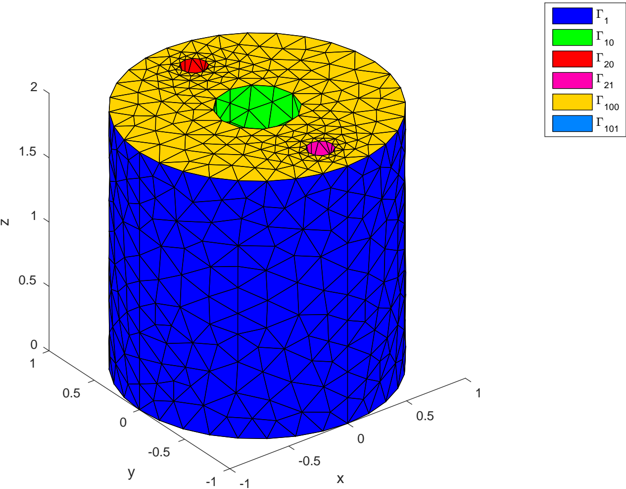
Boundaries of the mesh (cylinder3holes.geo)
