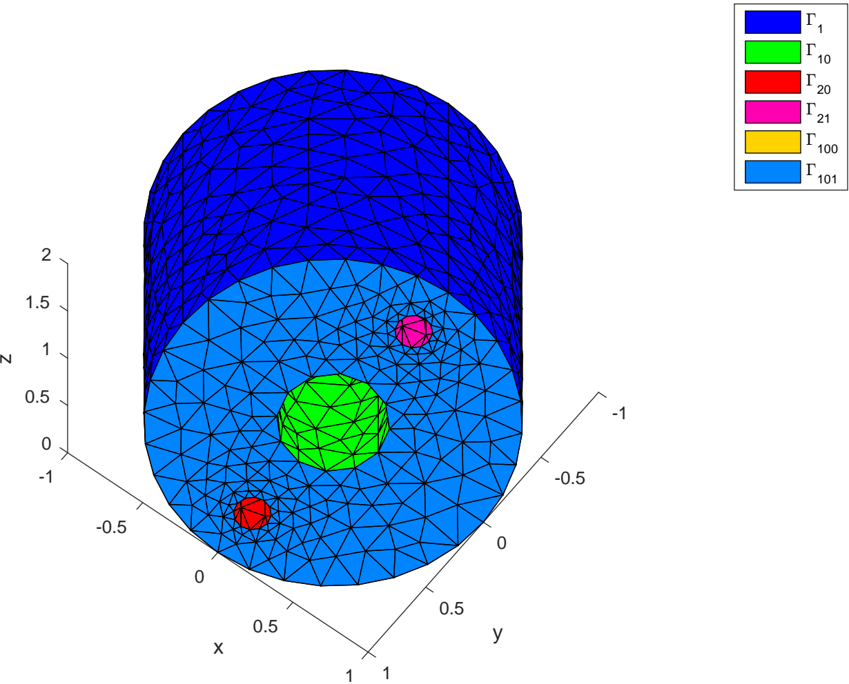
Boundaries of the mesh (cylinder3holes.geo)
