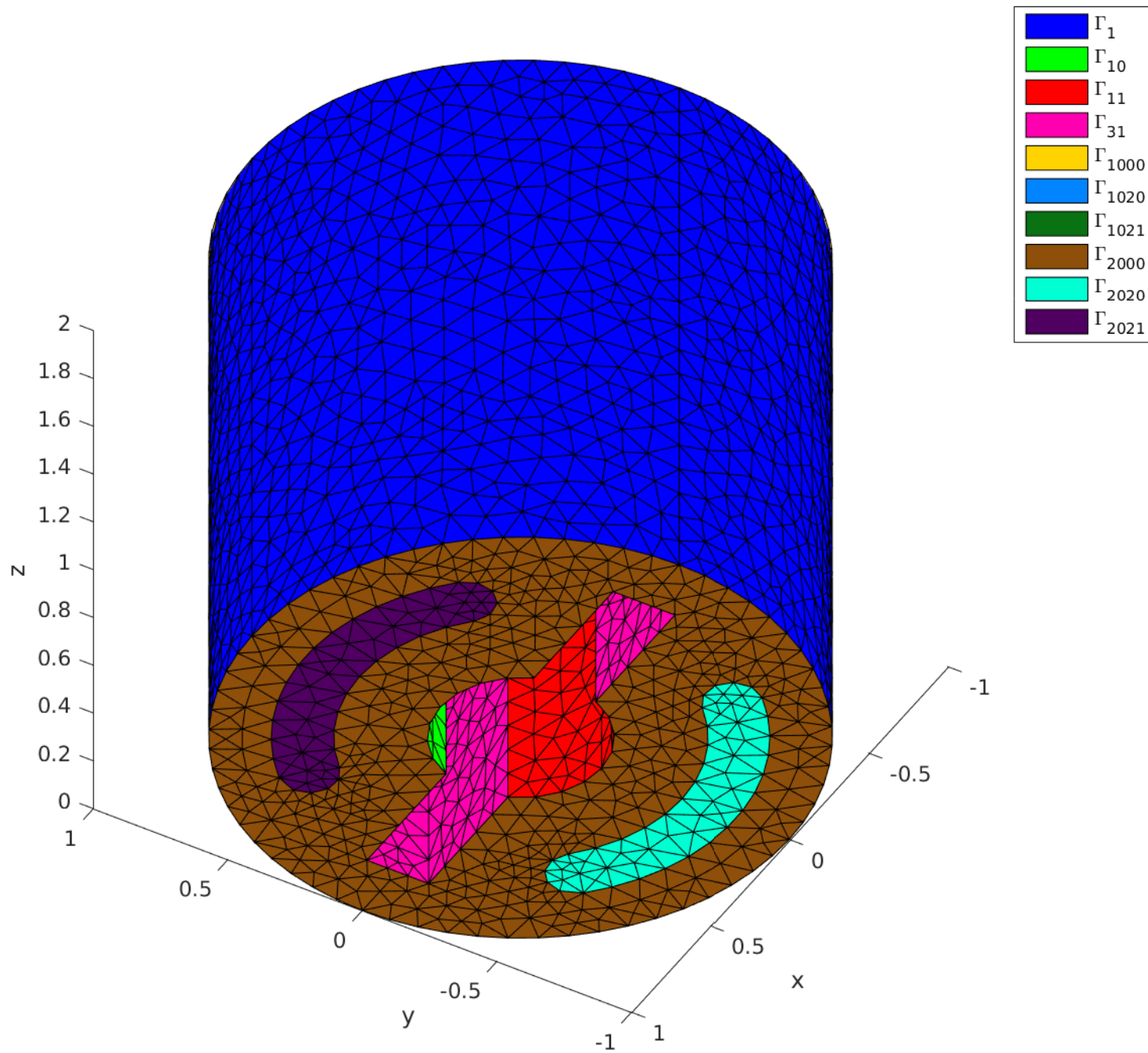
Mesh elements of 3d/cylinderkey-10.msh
