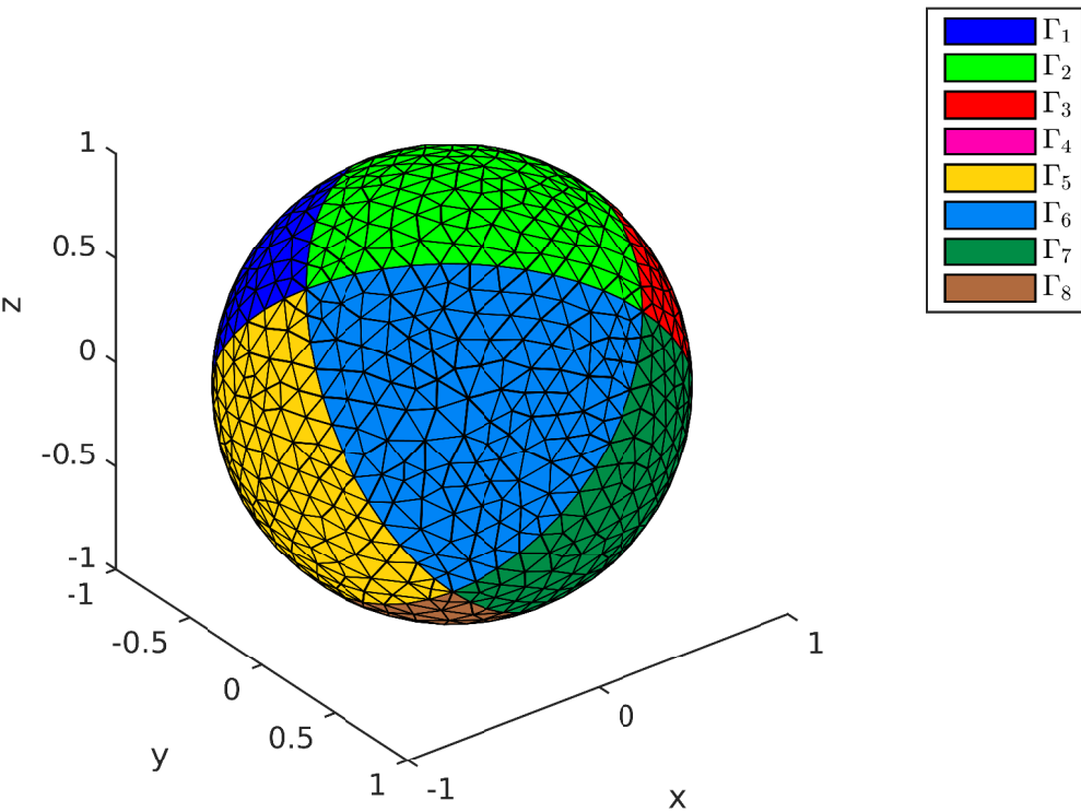
Mesh elements of 3d/sphere8.msh
