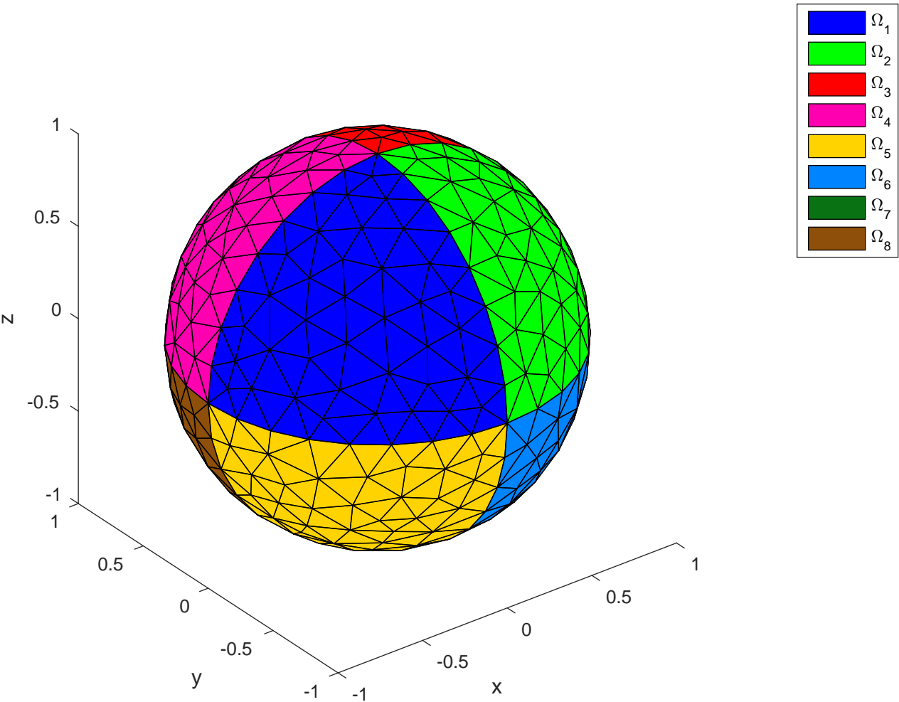
Domains of the 3D surface mesh (sphere8surf.geo)
