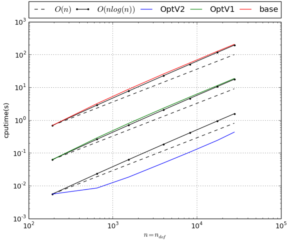
Figure 3.5: StiffElasAssembling3DP1 benchmark
