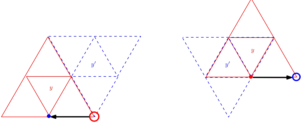
FIGURE 1. We illustrate the dichotomy given by the last paragraph of the proof of Proposition 4.1.8. We represent the data (y, (\widetilde{w}, \omega)) \in SP(x^*) by the alcove labeled by y and the dot (resp. circle) at \omega \in X^*(T)/X^0(T) when \widetilde{w} \cdot C_0 is lower (resp. upper) alcove (thus the left picture is the case where \widetilde{w} \cdot C_0 is upper alcove, and the right picture the case where \widetilde{w} \cdot C_0 is lower alcove). The starting pair (y, (\widetilde{w}, y\widetilde{w}^{-1}(0))) \in SP(x^*) is given by the red triangle (with vertexes labeled by the set W_{\mathrm{obv}}(y^*) ) and the source of the arrow (labeled by the obvious weight (\widetilde{w}, y\widetilde{w}^{-1}(0)) \in W_{\mathrm{obv}}(x^*) ). The dotted triangle represents the possible new specialization, while the tip of the arrow represents the new obvious weight.
