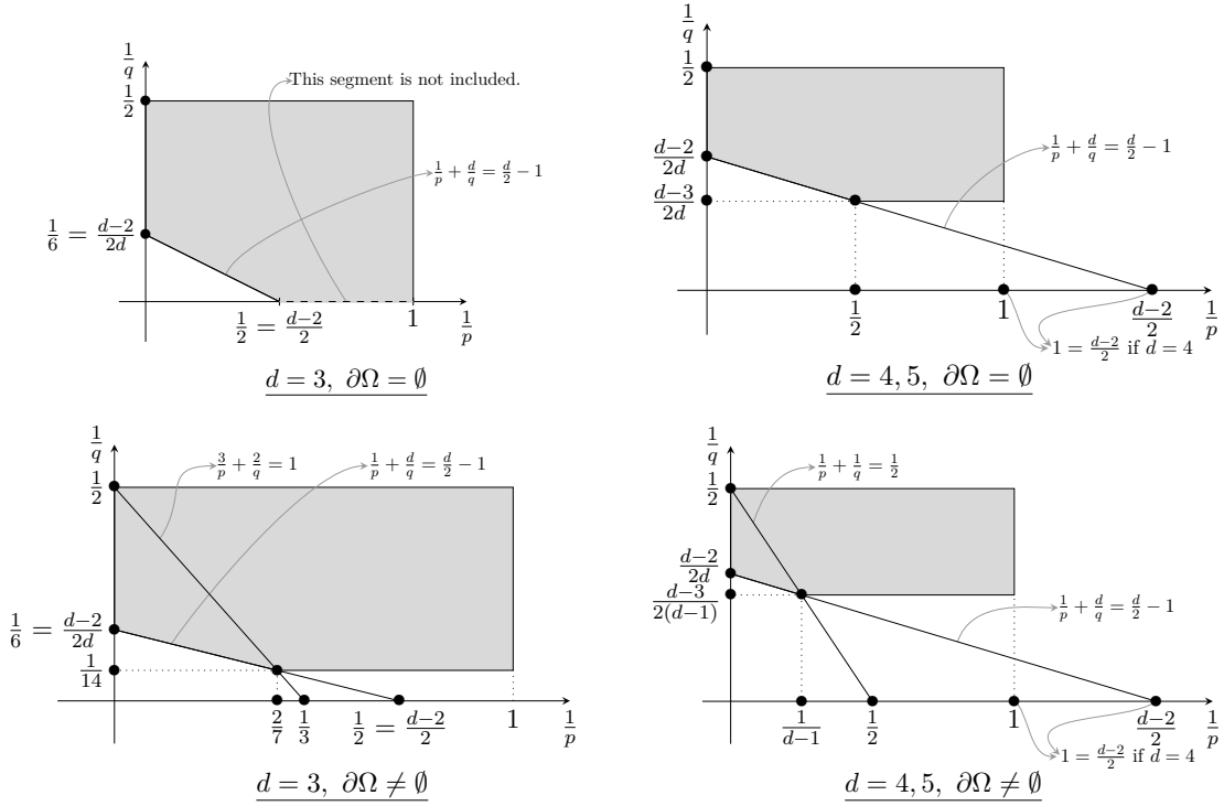
Figure 6.1: The local admissible exponents \Lambda_\Omega , in gray.
