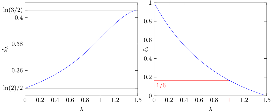
Figure 3.2 – The dimension and the speed of the \lambda -biased random walk on a Galton-Watson tree as functions of \lambda , for p_1 = p_2 = 1/2 .
