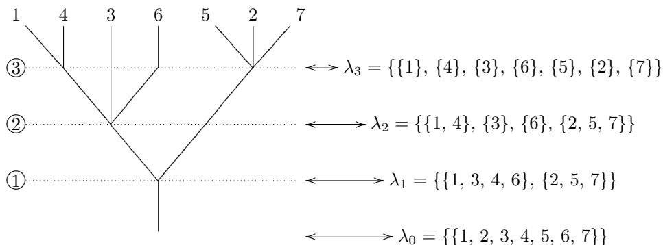
FIGURE 3. An example of the image of \Psi in the case \mathcal{P} = \mathcal{C}om .
