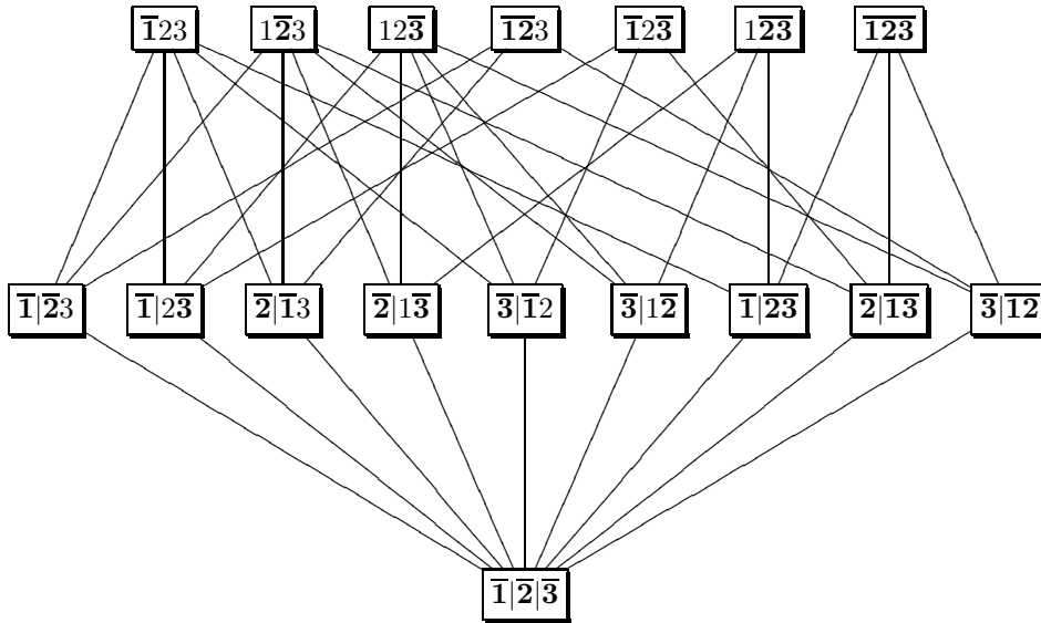
Figure 4: The poset \text{MII}_3^A
