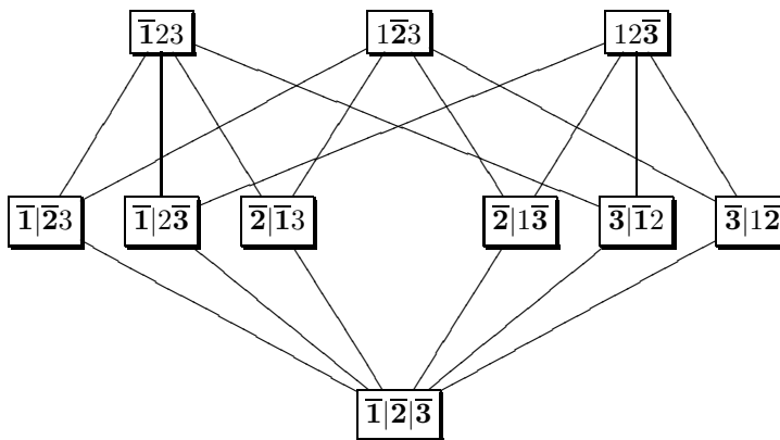
Figure 1: The poset \Pi_3^A
