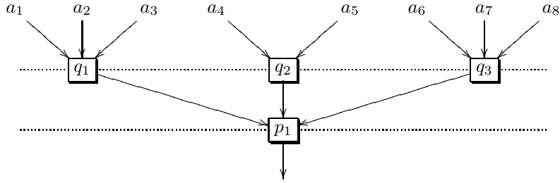
Figure 3: Example of composition of operations in (\mathcal{P} \circ \mathcal{Q})_8
